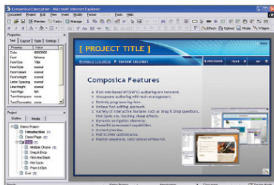
Authoring environment
