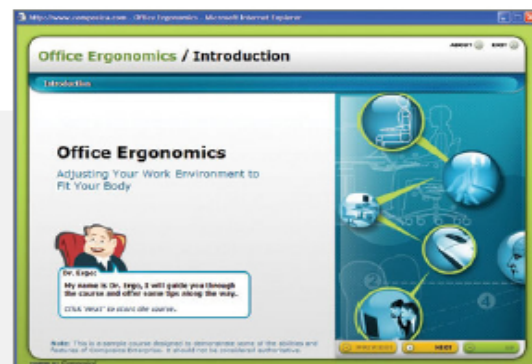
Sample course
